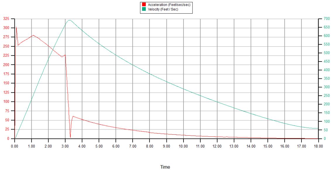
FIGURE 19:VELOCITY AND ACCELERATION DURING FIRST 30SEC OF FLIGHT
