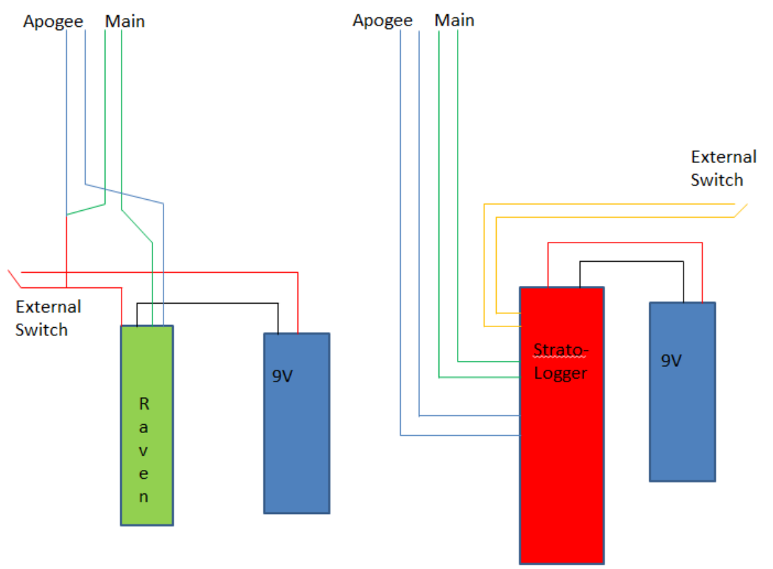
FIGURE 10: AVIONICS WIRING DIAGRAM
