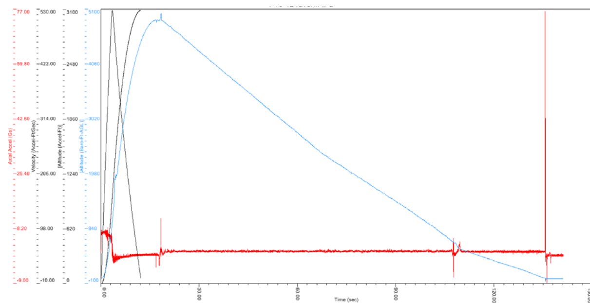
FIGURE 11: TEST FLIGHT FULL DATA
