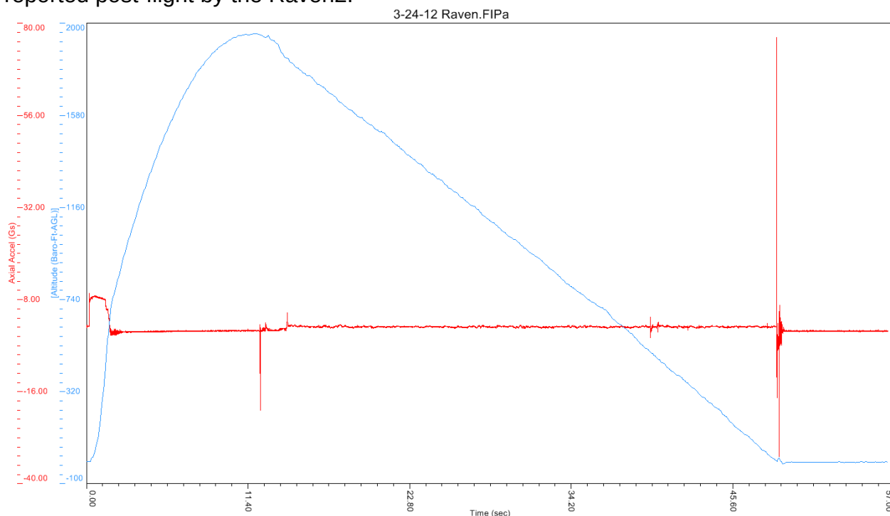
FIGURE 15: TEST FLIGHT FULL DATA
