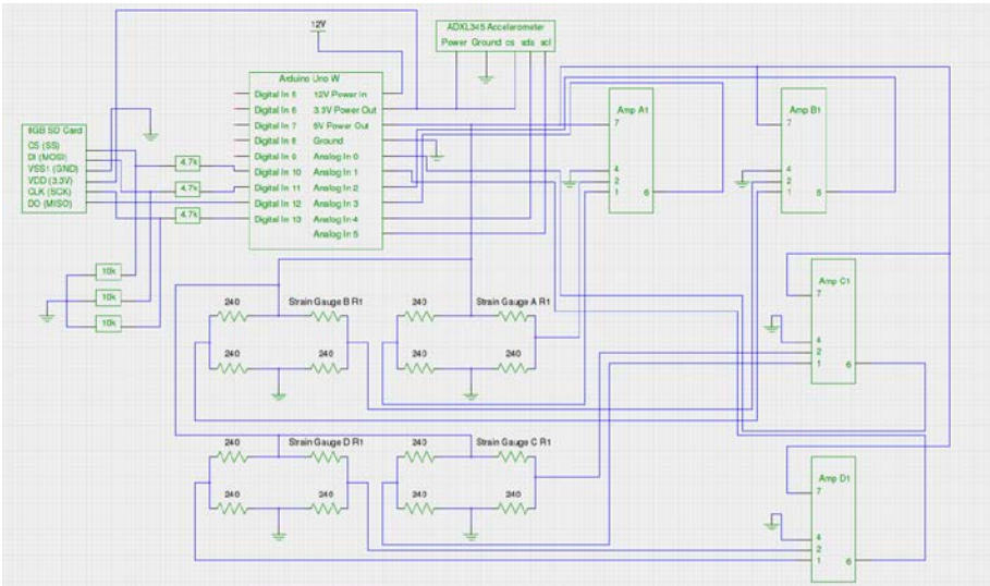
FIGURE 32: ARDUINO WIRING DIAGRAM
