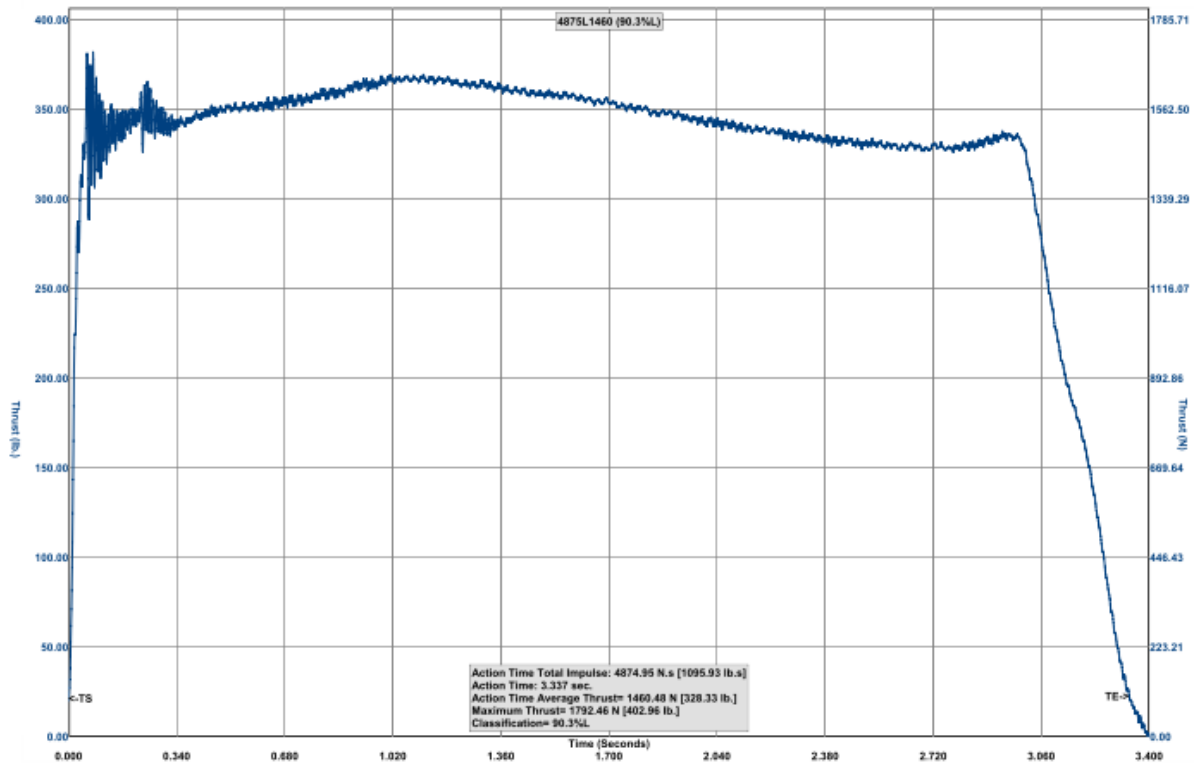
FIGURE 21:L1395 THRUST PROFILE
