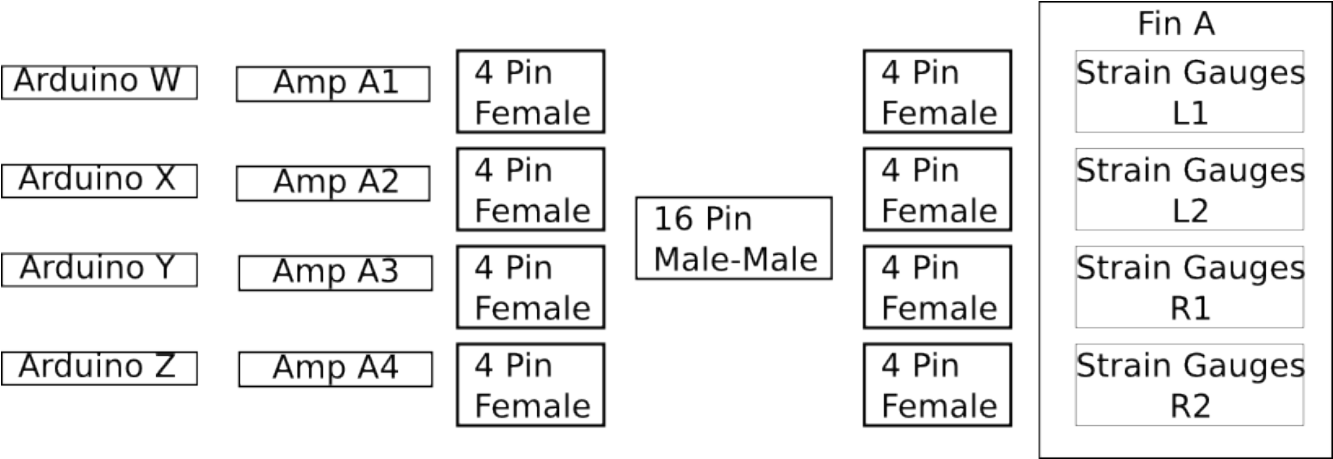
FIGURE 36: REMOTE SWITCH CIRCUIT DIAGRAM
