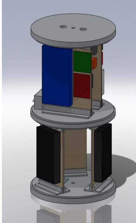
FIGURE 30: AVIONICS AND CAMERA BAY CAD MODEL VIEW 1
