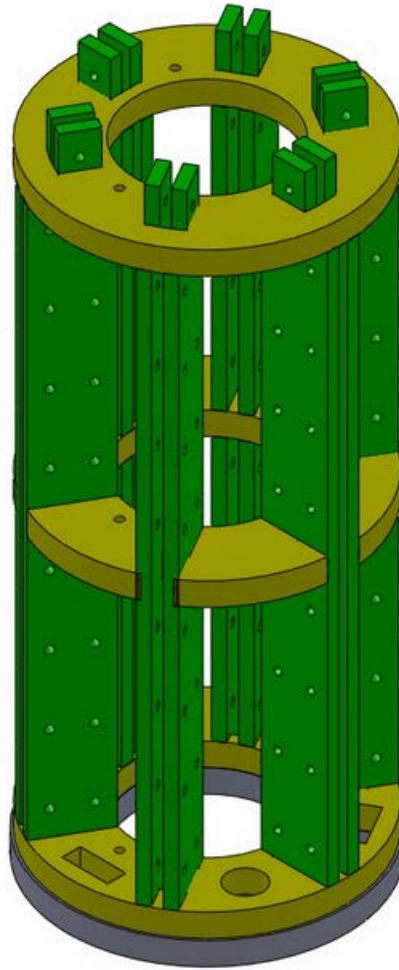
FIGURE 3: FIN HOLDER WITHOUT FINS
