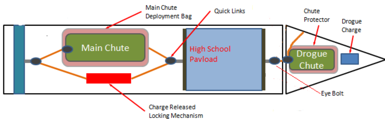
FIGURE 6:RECOVERY COMPONENT STACKING
