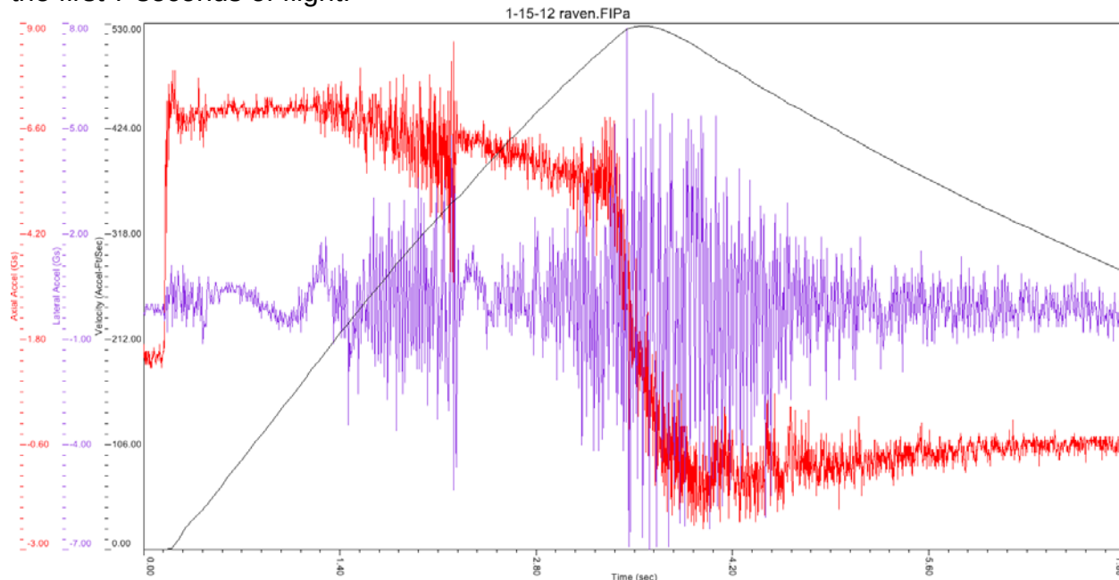
FIGURE 12: ACCELERATION AND VELOCITY FOR FIRST 7 SECONDS OF FULL SCALE LAUNCH
