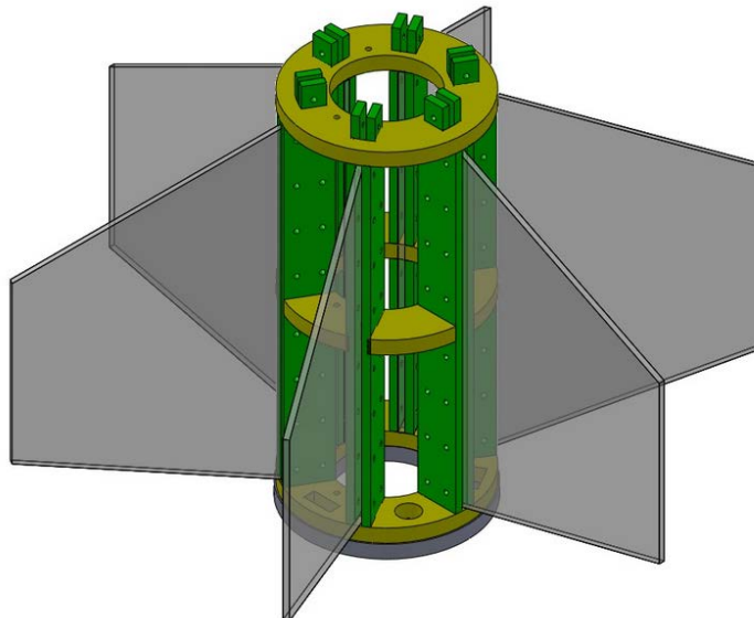
FIGURE 4: FIN HOLDER WITH FINS
