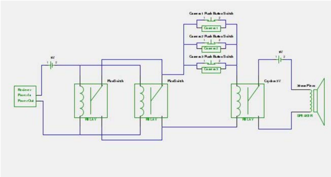
FIGURE 33: ARUINO WIRING DIAGRAM
