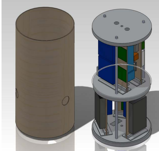
FIGURE 9: AVIONICS BAY CONFIGURATION
