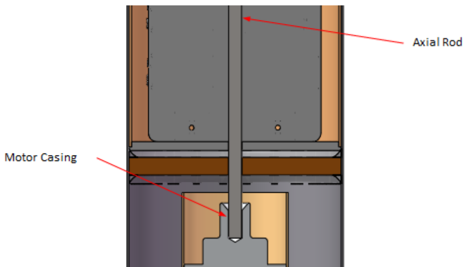
FIGURE 5: MOTOR RETENTION
