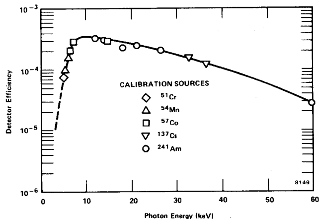
Fig. 21.3. Typical Si(Li) Detector Efficiency Curve (using 10-mil Mylar absorber).
