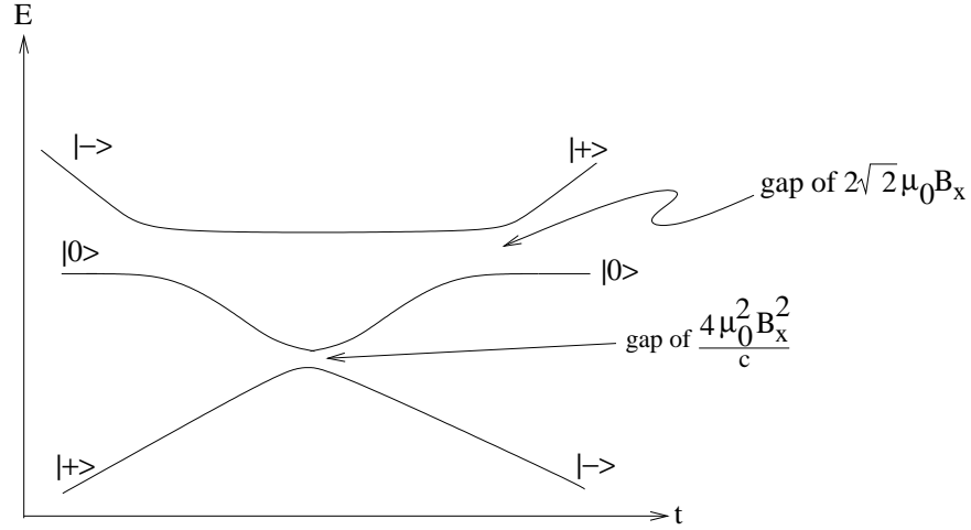
Figure 3: Sketch of the evolution of the energy levels.
