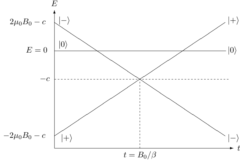
Figure 2: The energy levels of the system without B_x .
