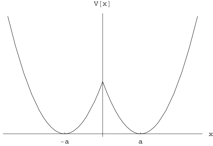
Figure 1: Double well potential
