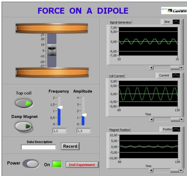
Figure 2: LabVIEW application Front Panel
