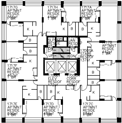
SEVENTEENTH FLOOR
