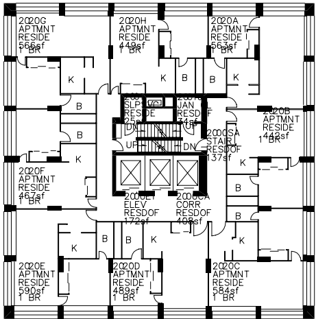
TWENTIETH FLOOR
