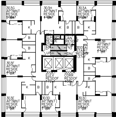
THIRD FLOOR
