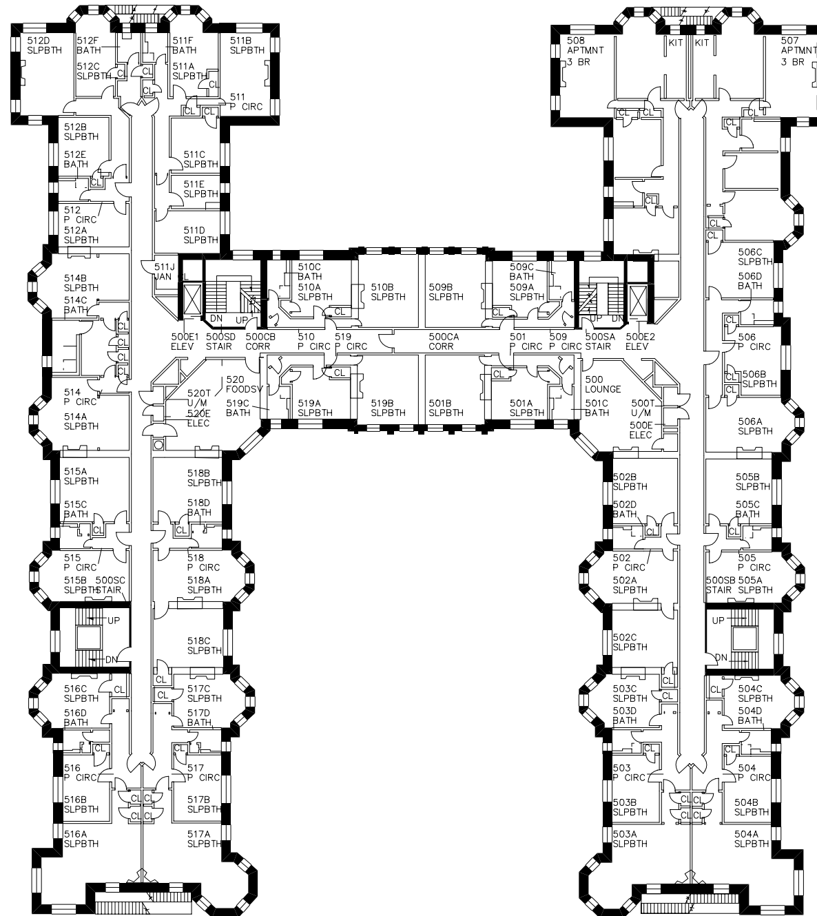
FIFTH FLOOR
