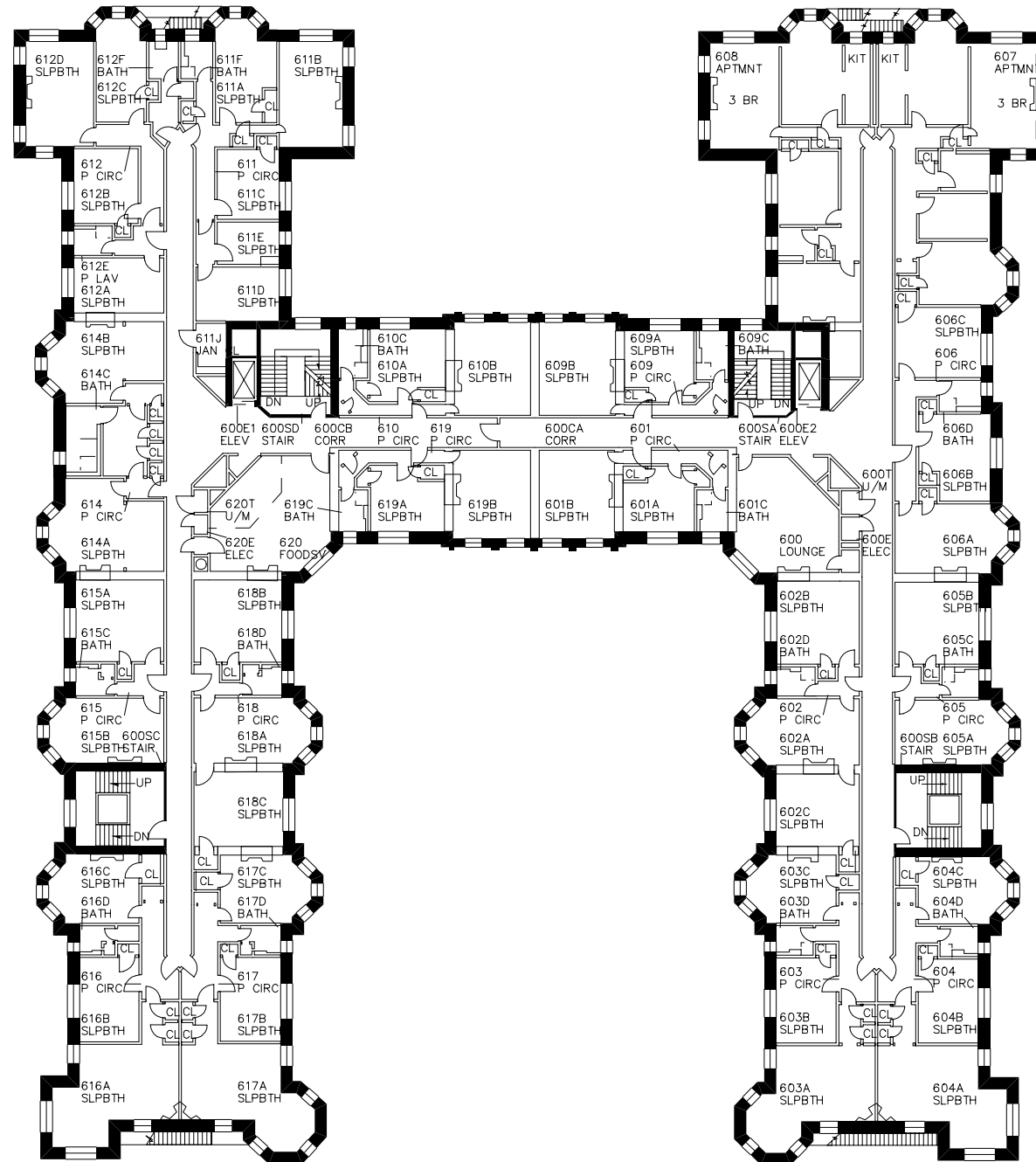
SIXTH FLOOR
