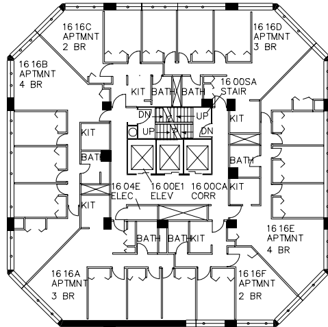
SIXTEENTH FLOOR
