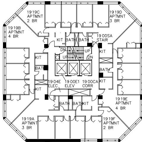
NINETEENTH FLOOR
