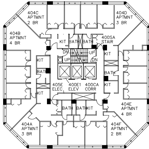
FOURTH FLOOR
