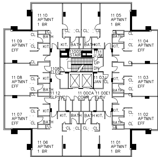
ELEVENTH FLOOR
