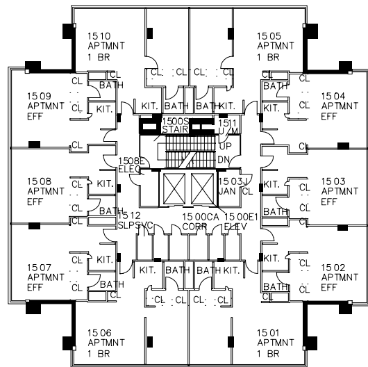
FIFTEENTH FLOOR
