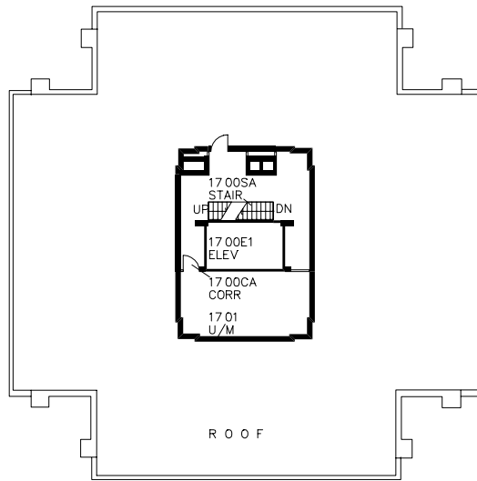
SEVENTEENTH FLOOR AND ROOF
