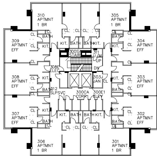
THIRD FLOOR
