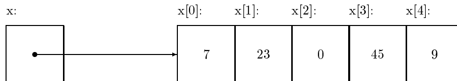
Figure 3: Box-and-pointer diagram of arrays: static int x[5] = {7,23,0,45,9};
