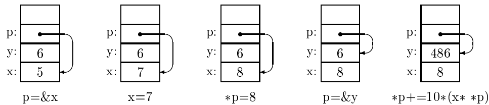
Figure 2: Memory diagram with pointers—the example program
