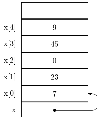
Figure 4: Memory diagram of arrays
