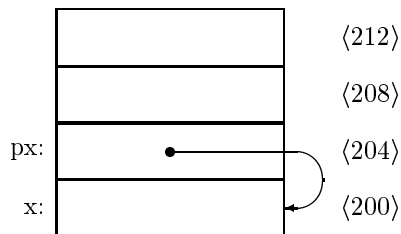
Figure 1: Memory diagram with pointers. The memory addresses are given by \langle n \rangle
