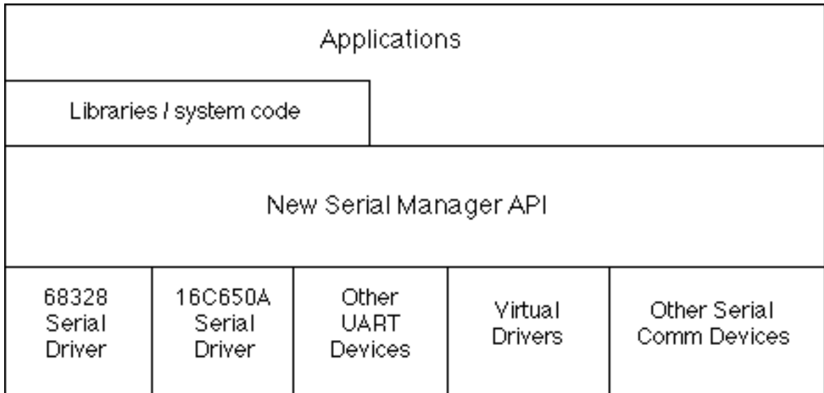
Figure 9.2 Serial Communications Architecture with New Serial Manager
