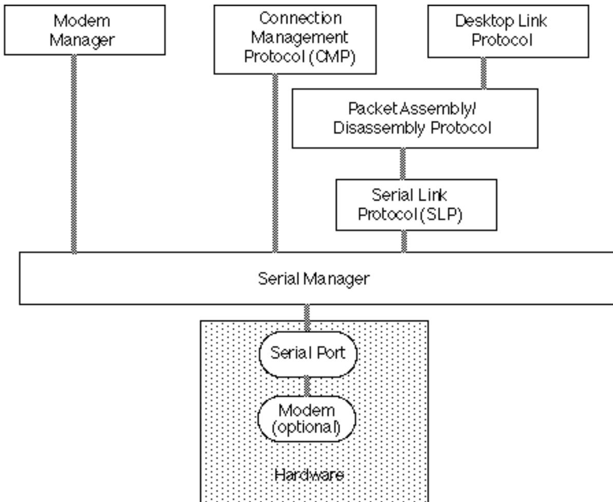
Figure 9.1 Palm OS Serial Communications Architecture
