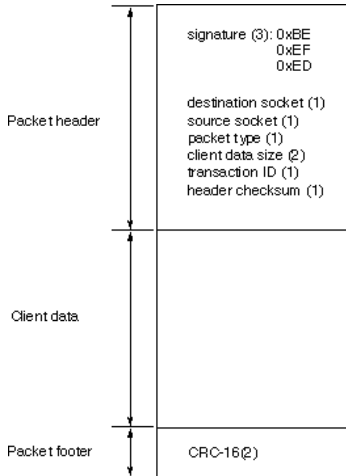
Figure 9.3 Structure of a Serial Link Packet
