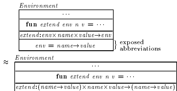
Figure 20: Exposing information for a type
