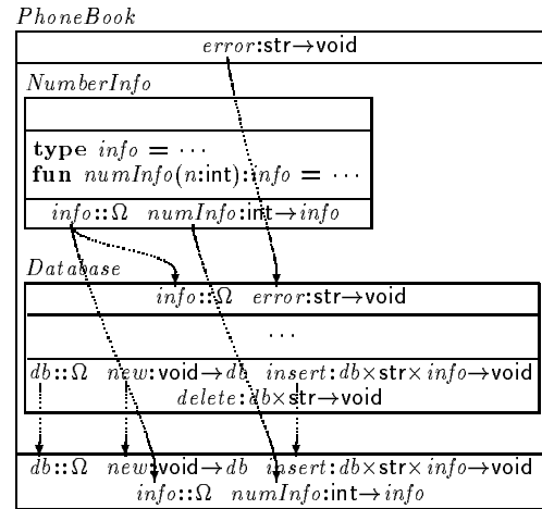
Figure 2: Linking units to form a compound unit
