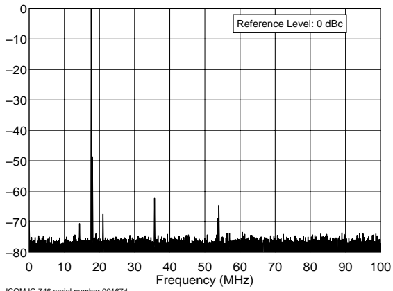
ICOM IC-746 serial number 001674 18.1 MHz Band, Spectral Purity, 100 W F:\SHARED\PROD_REV\TESTS\IC746\IC746S17.TXT
