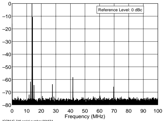
ICOM IC-746 serial number 001674 14.0 MHz Band, Spectral Purity, 100 W F:\SHARED\PROD_REV\TESTS\IC746\IC746S20.TXT
