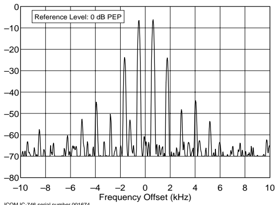
ICOM IC-746 serial number 001674 50.200 MHz, Transmit IMD, 100 W F:\SHARED\PROD_REV\TESTS\IC746\IC746I6M.TXT
