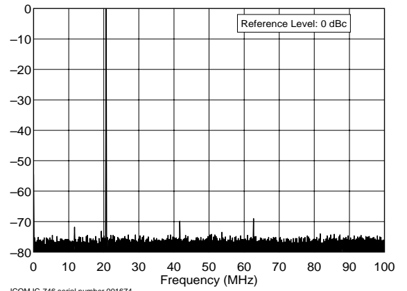
ICOM IC-746 serial number 001674 21.0 MHz Band, Spectral Purity, 100 W F:\SHARED\PROD_REV\TESTS\IC746\IC746S15.TXT
