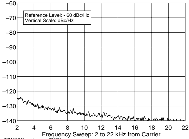
ICOM IC-746 serial number 001674 3.520 MHz, Phase Noise, 100 W F:\SHARED\PROD_REVTESTS\IC746\IC746P80.TXT
