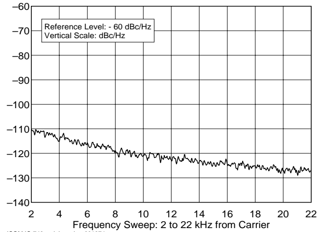
ICOM IC-746 serial number 001674 144.020 MHz, Phase Noise, 100 W F:\SHARED\PROD_REVTESTS\IC746\IC746P2M.TXT
