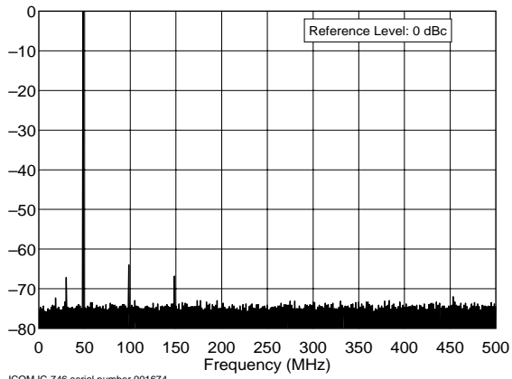
ICOM IC-746 serial number 001674 50.0 MHz Band, Spectral Purity, 100 W F:\SHARED\PROD_REV\TESTS\IC746\IC746S6M.TXT
