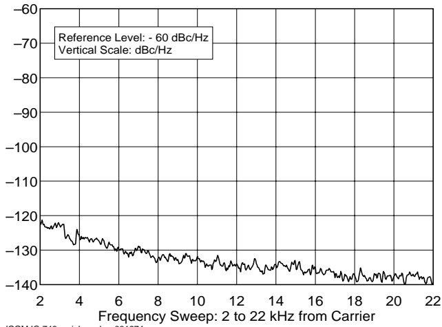
ICOM IC-746 serial number 001674 14.020 MHz, Phase Noise, 100 W F:\SHARED\PROD_REVTESTS\IC746\IC746P20.TXT
