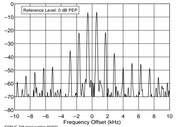
ICOM IC-746 serial number 001674 144.200 MHz, Transmit IMD, 100 W F:\SHARED\PROD_REV\TESTS\IC746\IC746I2M.TXT
