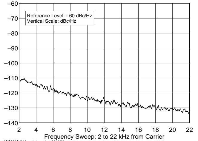
ICOM IC-746 serial number 001674 50.020 MHz, Phase Noise, 100 W F:\SHARED\PROD_REVTESTS\IC746\IC746P6M.TXT
