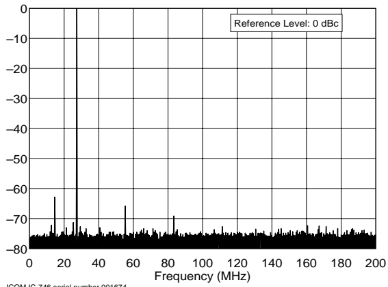
ICOM IC-746 serial number 001674 28.0 MHz Band, Spectral Purity, 100 W F:\SHARED\PROD_REV\TESTS\IC746\IC746S10.TXT
