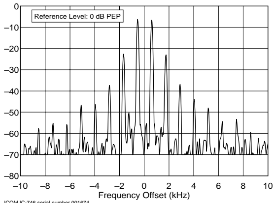
ICOM IC-746 serial number 001674 28.350 MHz, Transmit IMD, 100 W F:\SHARED\PROD_REV\TESTS\IC746\IC746I10.TXT
