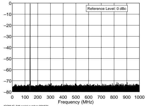
ICOM IC-746 serial number 001674 144.0 MHz Band, Spectral Purity, 100 W F:\SHARED\PROD_REV\TESTS\IC746\IC746S2M.TXT
