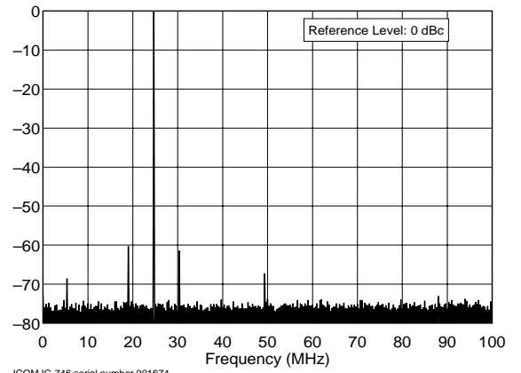
ICOM IC-746 serial number 001674 24.9 MHz Band, Spectral Purity, 100 W F:\SHARED\PROD_REV\TESTS\IC746\IC746S12.TXT
