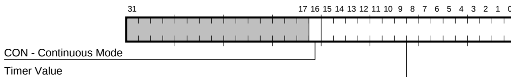
Figure 3–23 CSR11 Register Bit Fields
