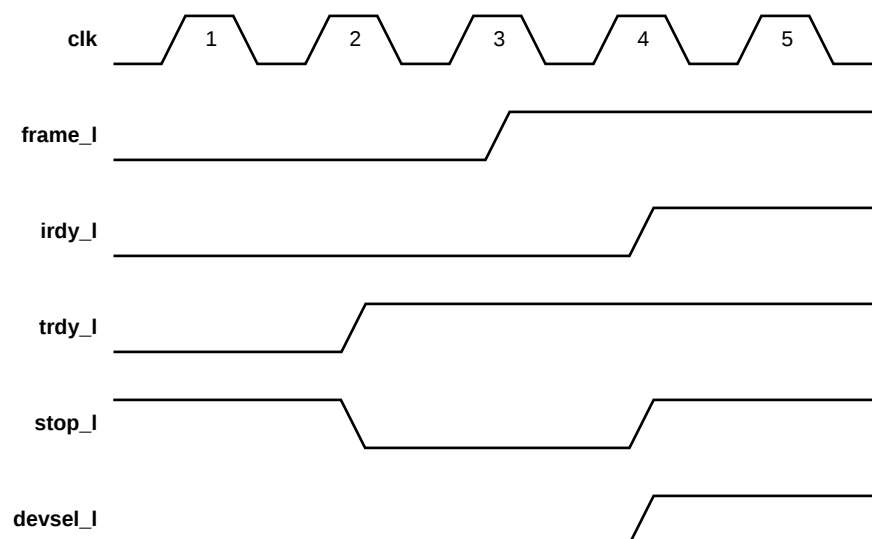
Figure 5-13 Target Retry
