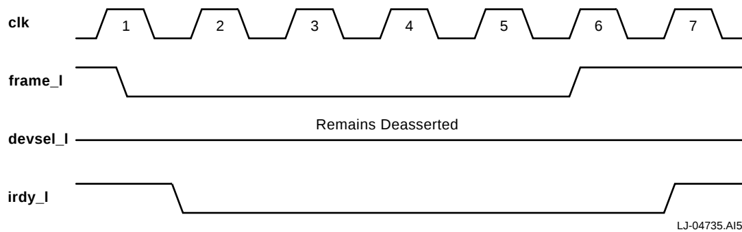
Figure 5–10 Master Abort
