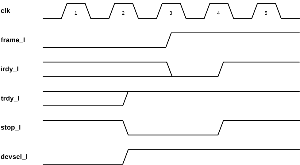
Figure 5–11 Target Abort
