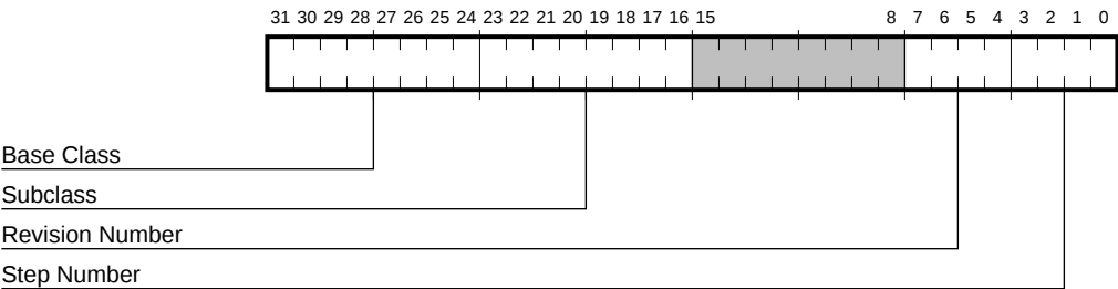
Figure 3–3 CFRV Register Bit Fields
