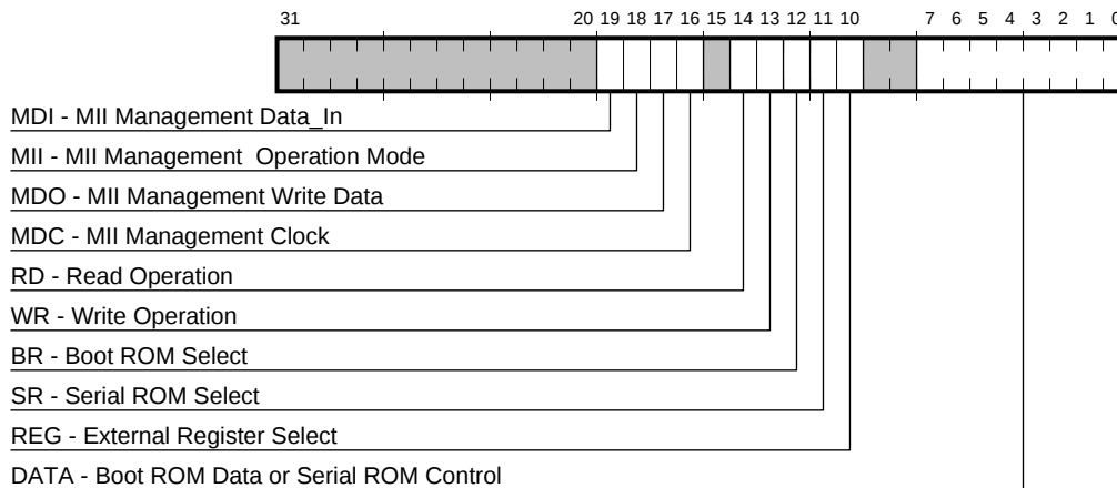
Figure 3–21 CSR9 Register Bit Fields
