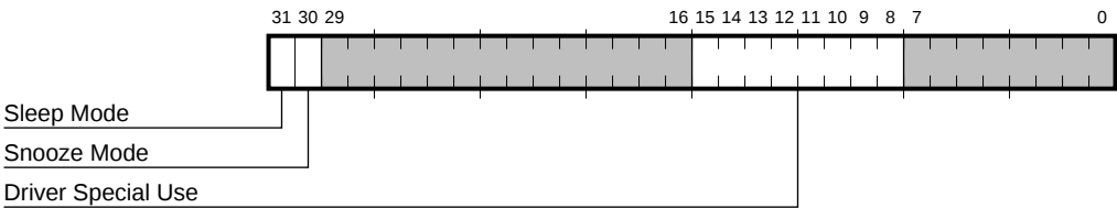
Figure 3–11 CFDD Register Bit Fields
