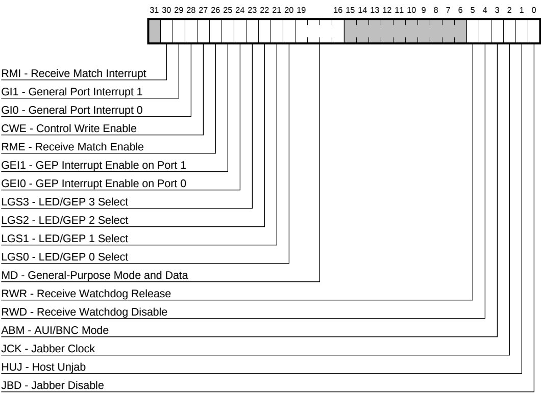
Figure 3–27 CSR15 Register Bit Fields
