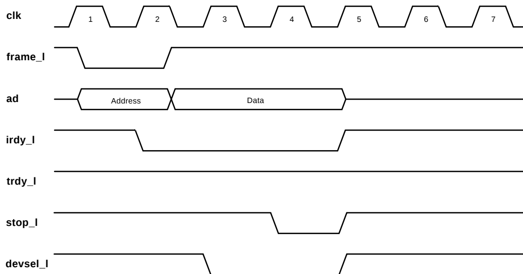
Figure 5–8 21142-Initiated Retry Cycle
