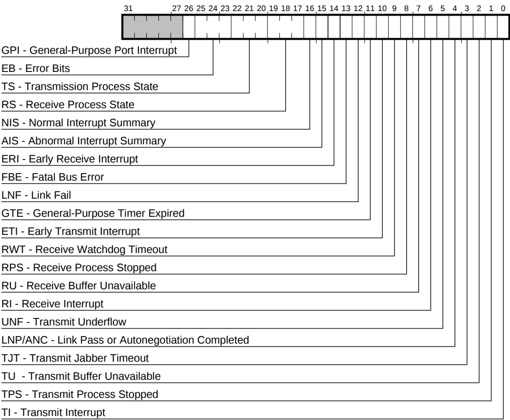
Figure 3–17 CSR5 Register Bit Fields
