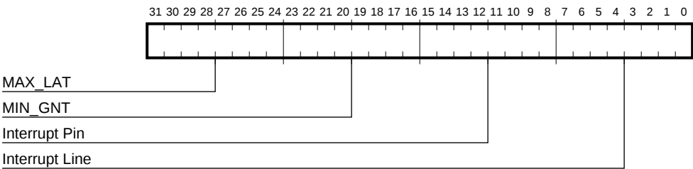
Figure 3–10 CFIT Register Bit Fields
