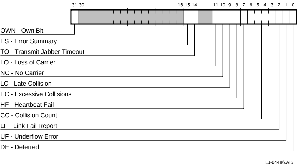
Figure 4–8 TDES0 Bit Fields
