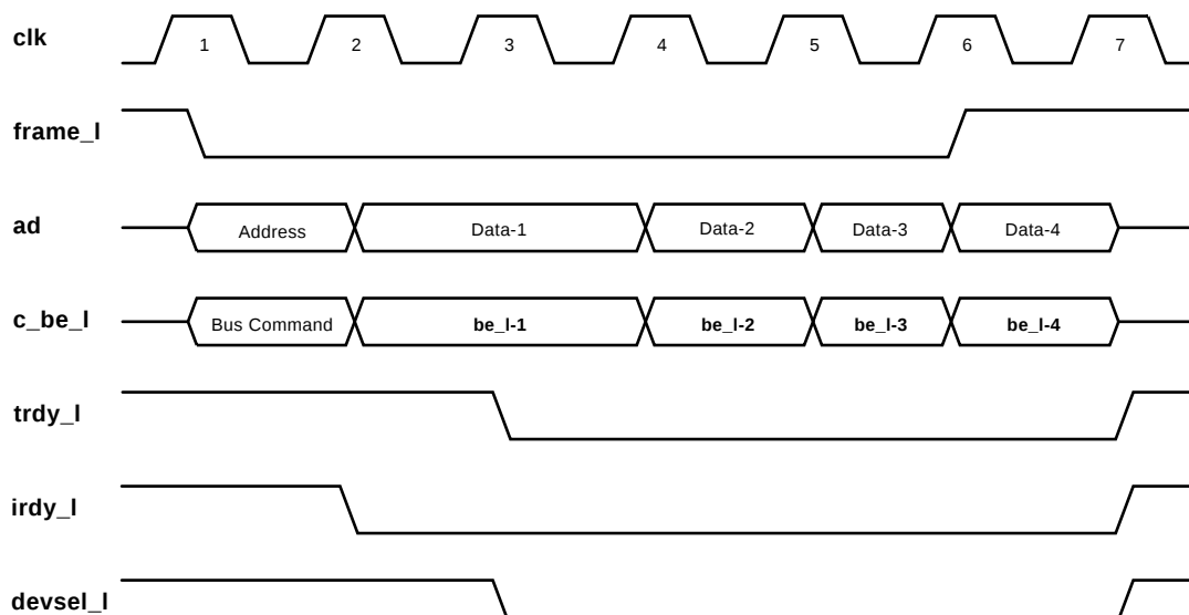
Figure 5–6 Memory Write Cycle
