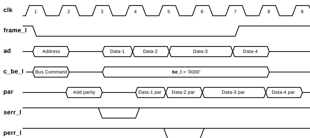
Figure 5-14 Parity Operation
