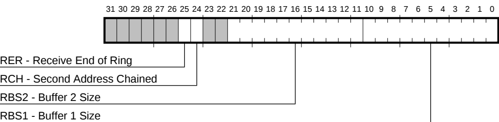
Figure 4–4 RDES1 Bit Fields
