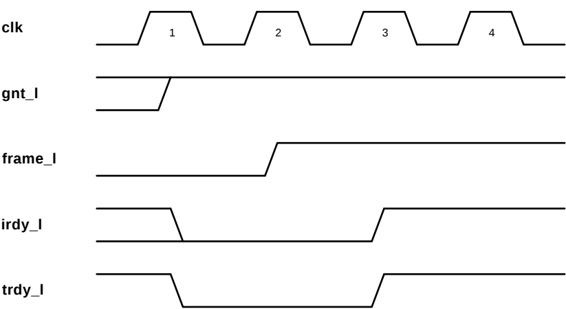
Figure 5–9 Normal Completion
