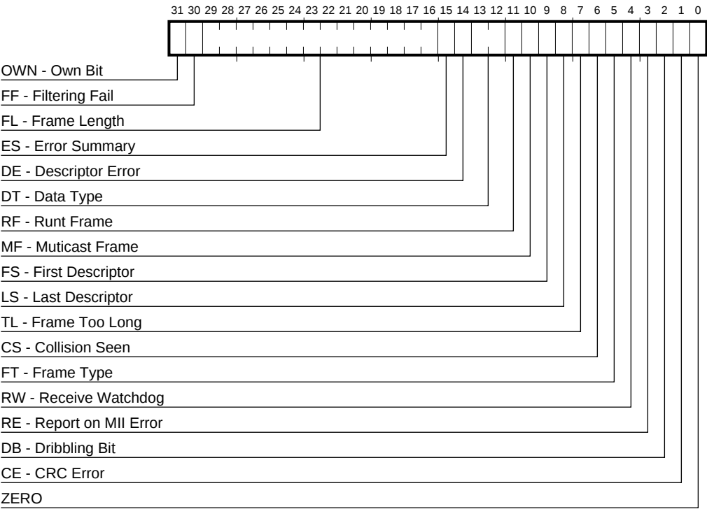
Figure 4-3 RDES0 Bit Fields
