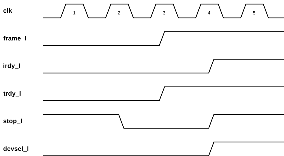
Figure 5–12 Target Disconnect
