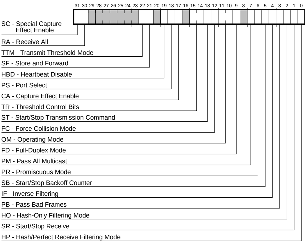
Figure 3–18 CSR6 Register Bit Fields
