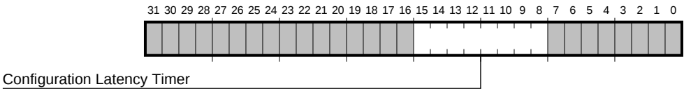
Figure 3–4 CFLT Register Bit Field
