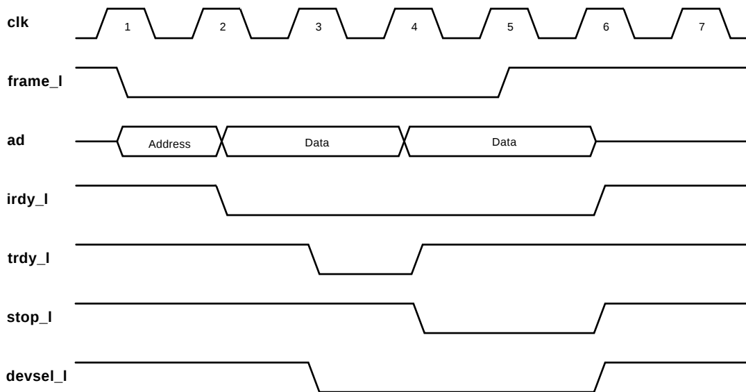
Figure 5–7 21142-Initiated Disconnect Cycle
