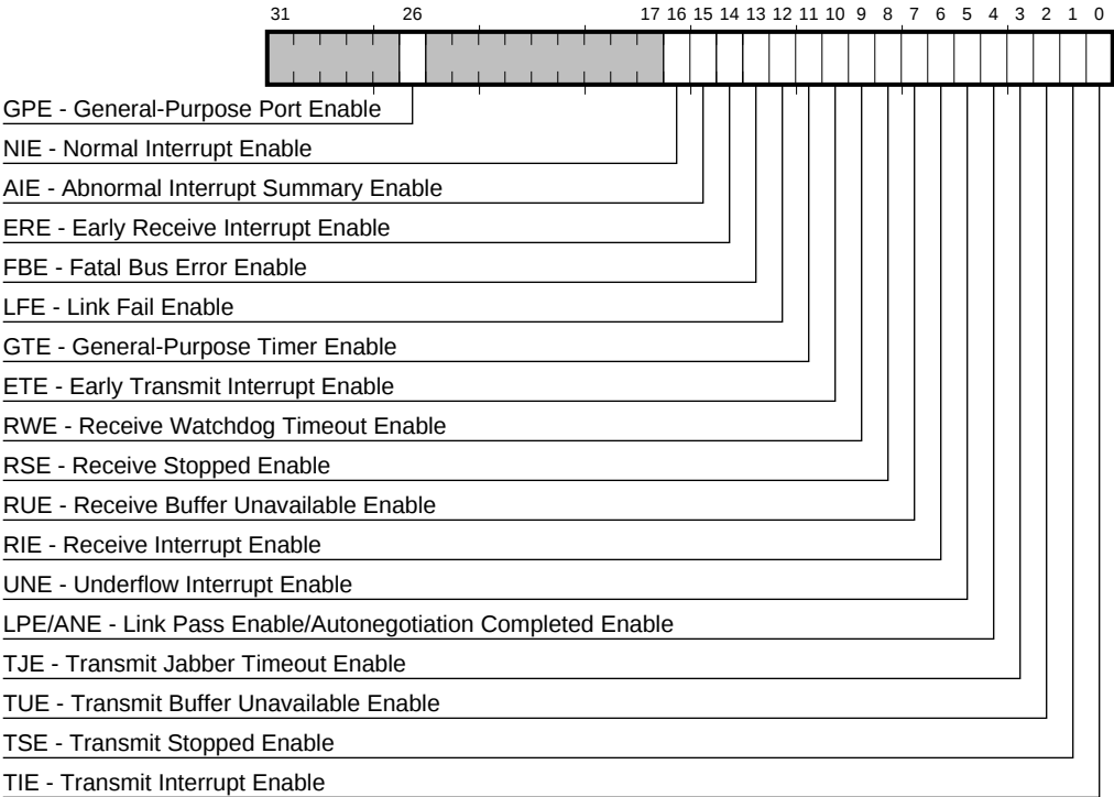
Figure 3–19 CSR7 Register Bit Fields
