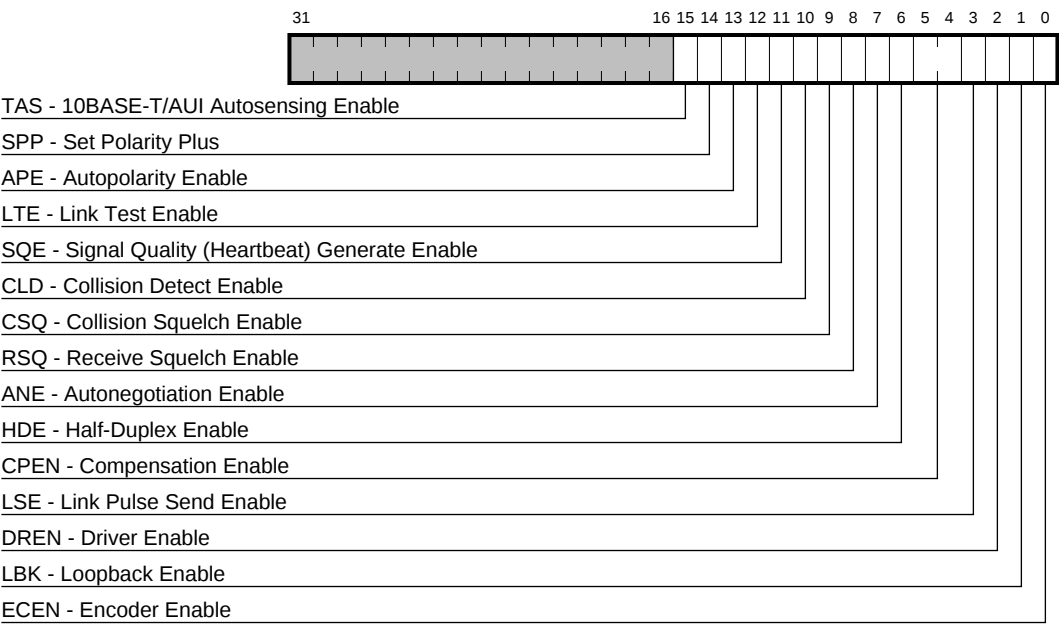
Figure 3–26 CSR14 Register Bit Fields
