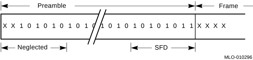
Figure 6-2 Preamble Recognition Sequence in 10BASE-T or AUI Mode
