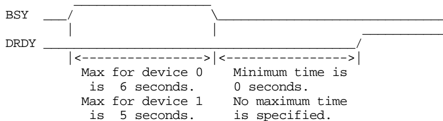
Figure 7 - BSY and DRDY timing for Diagnostic command
