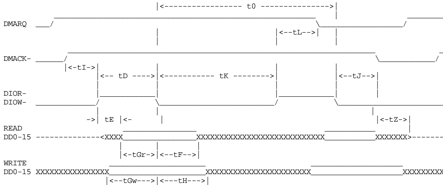
Figure 12 - Multiword DMA Data Transfer (Part 1 of 2)
