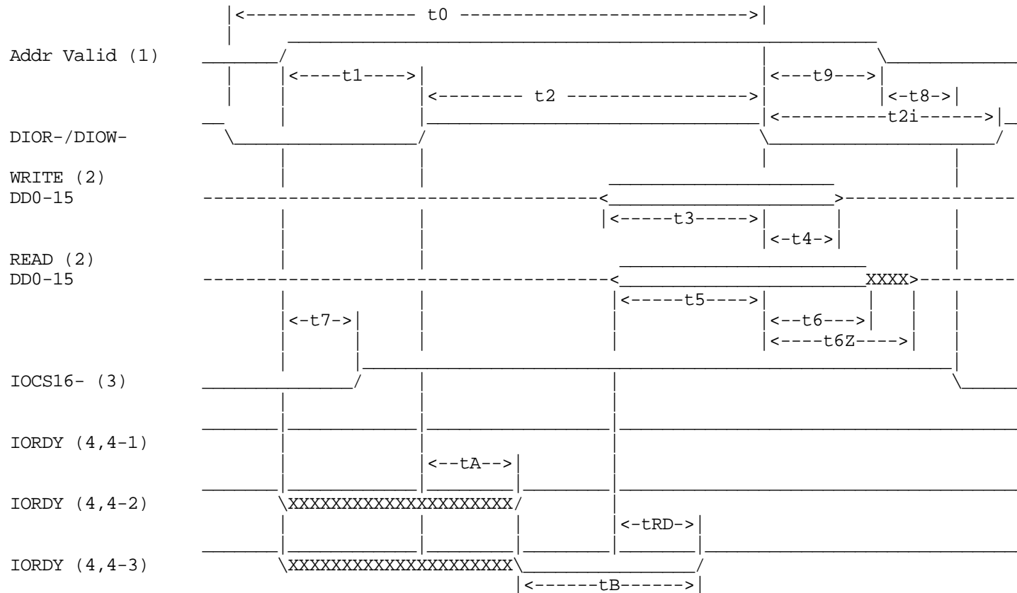
FIGURE 10 - PIO Data Transfer to/from Device (Part 1 of 2)
