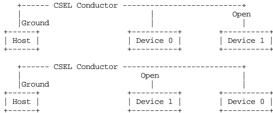
Figure 4 - Cable Select Example
