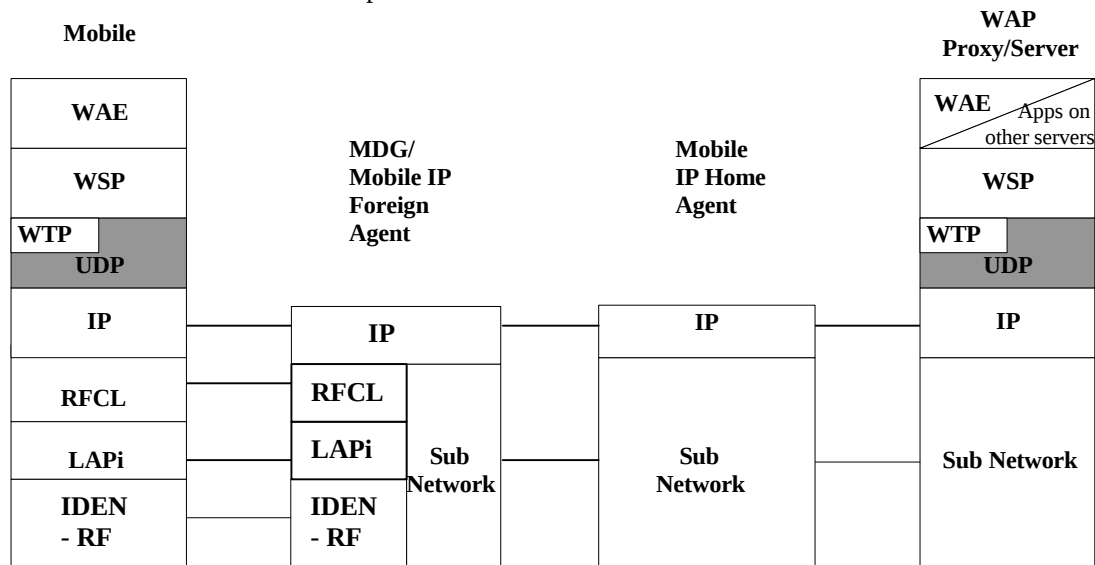
Figure 5.22: WTP over iDEN Packet Data
