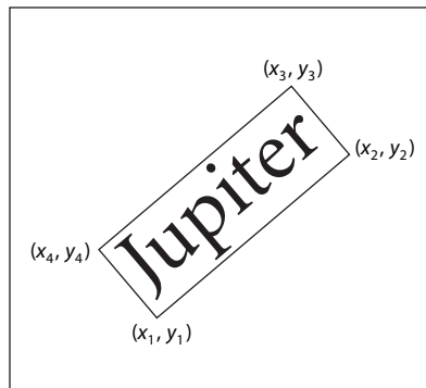
FIGURE 7.5 QuadPoints specification
