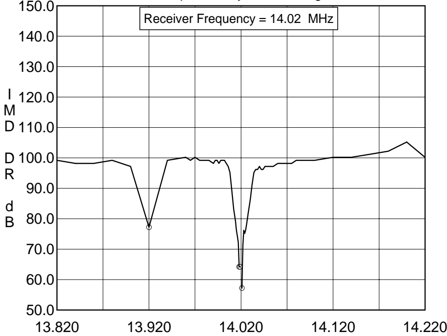
Swept IMD Dynamic Range
