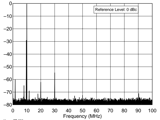
Yaesu FT-920 10.1 MHz Band, Spectral Purity, 100 W
