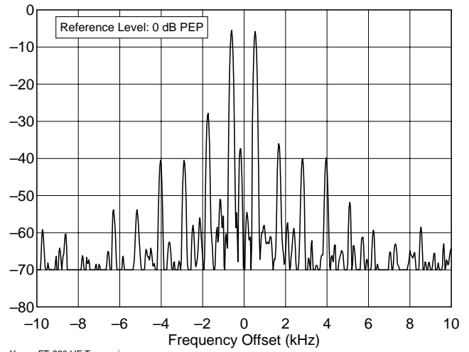
Yaesu FT-920 HF Transceiver 10.120 MHz, Transmit IMD, 100 W
