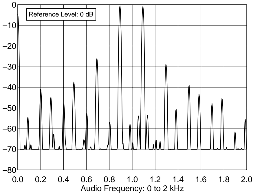
Yaesu FT-920 HF Transceiver 14.200 MHz, AGC Fast, In-Band Receiver IMD
