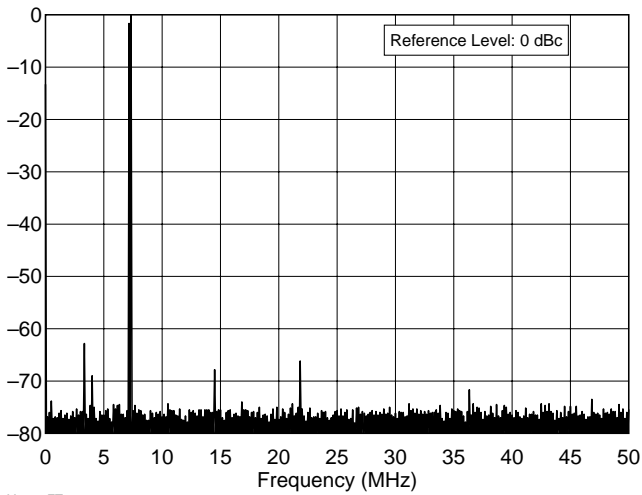
Yaesu FT-920 7.0 MHz Band, Spectral Purity, 100 W
