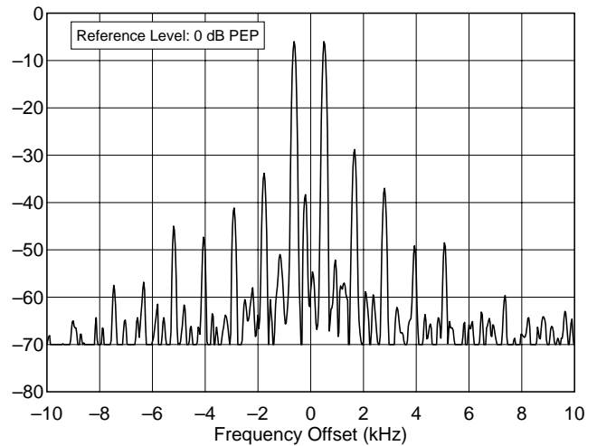
Yaesu FT-920 HF Transceiver 18.120 MHz, Transmit IMD, 100 W
