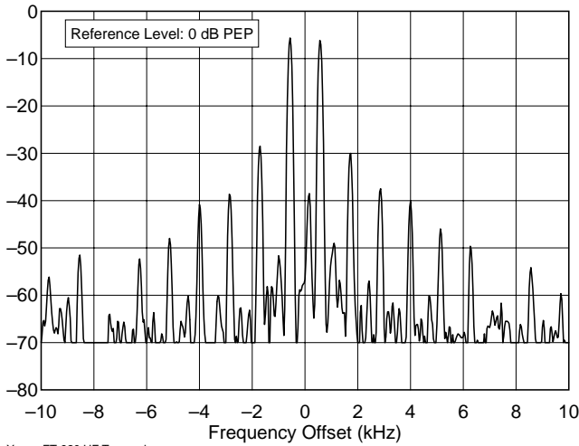
Yaesu FT-920 HF Transceiver 1.850 MHz, Transmit IMD, 100 W
