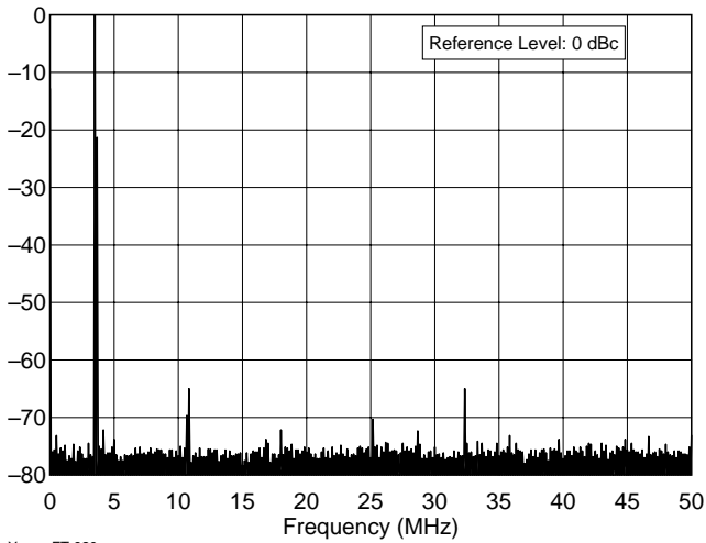
Yaesu FT-920 3.5 MHz Band, Spectral Purity, 100 W
