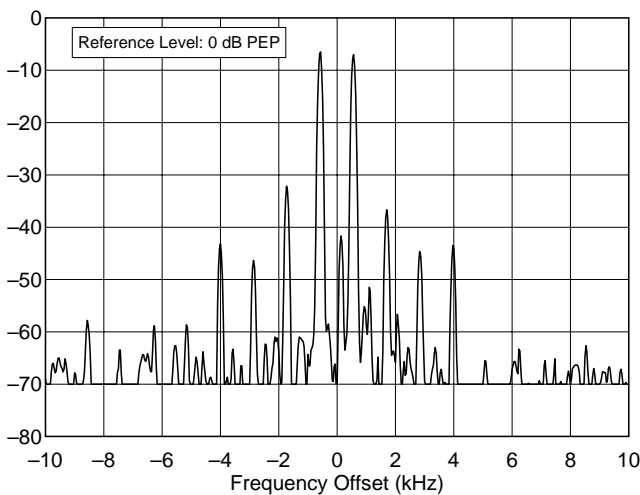
Yaesu FT-920 HF Transceiver 7.250 MHz, Transmit IMD, 100 W
