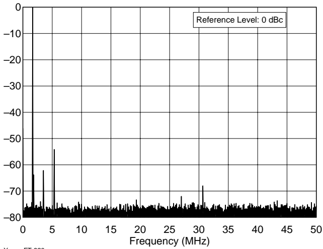
Yaesu FT-920 1.8 MHz Band, Spectral Purity, 100 W
