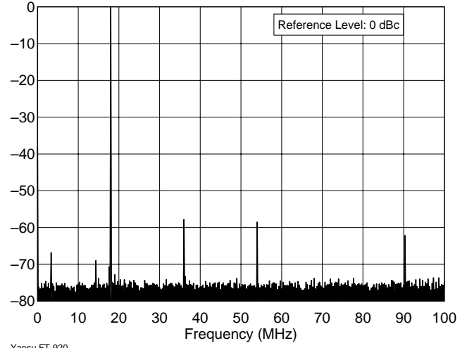
Yaesu FT-920 18.1 MHz Band, Spectral Purity, 100 W
