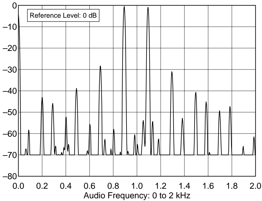
Yaesu FT-920 HF Transceiver 14.200 MHz, AGC Slow, In-Band Receiver IMD
