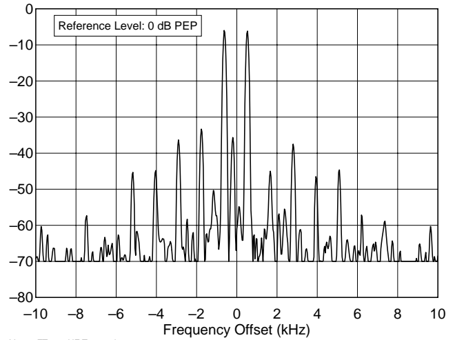
Yaesu FT-920 HF Transceiver 14.250 MHz, Transmit IMD, 100 W
