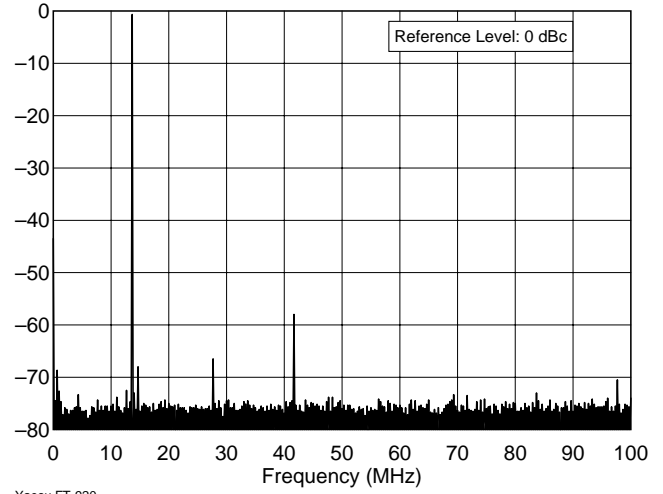
Yaesu FT-920 14.0 MHz Band, Spectral Purity, 100 W
