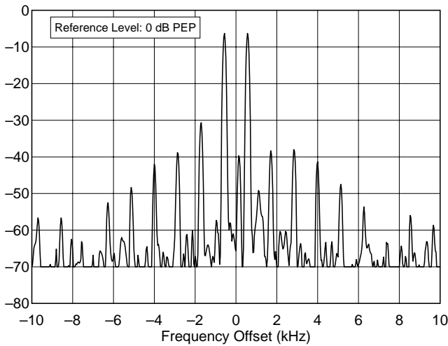
Yaesu FT-920 HF Transceiver 3.900 MHz, Transmit IMD, 100 W
