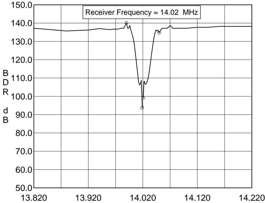
Swept Blocking Dynamic Range
