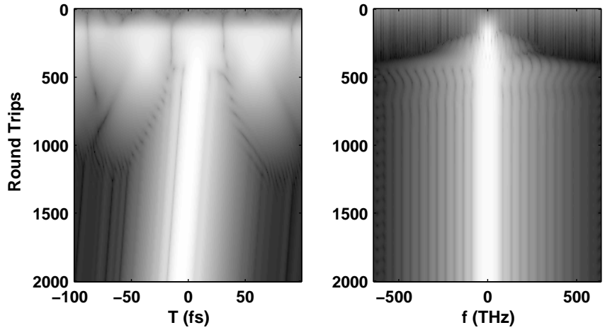
Figure 2-3: Evolution of model laser starting from noise, shown on a log scale. The field intensity as a function of time is on the left, with the power spectral density shown on the right. The pulse does not exactly follow our moving window because of nonlinear effects shifting the spectrum from our assumed center frequency.
