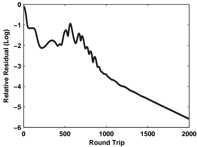
Figure 2-4: Convergence of dynamic cavity evolution. Once the initial transients die, the convergence of the pulse shaping mechanism is linear.
