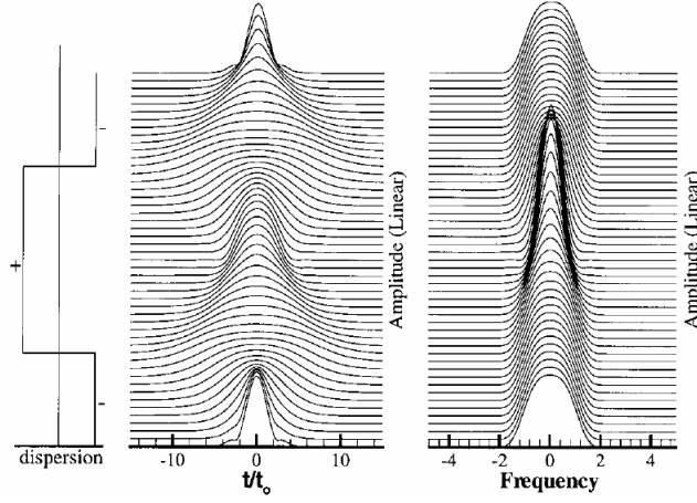
Figure 2-2: Illustration of the pulseshaping mechanism of a dispersion managed soliton laser over one round-trip. Adapted from [13].
