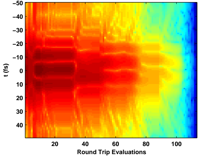
Figure 4-4: The sequence of residuals produced by the direct solver as a function of the number of round trip evaluations, log scaled.
