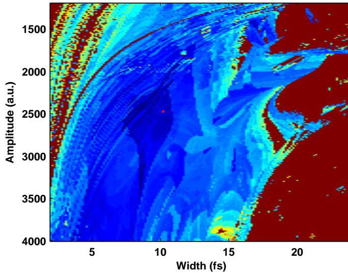
Figure 4-3: Convergence map of Newton-Krylov solver for Gaussian starting iterates of various widths and amplitudes for a ten femtosecond laser model (chosen for its quick convergence). The darker colors represent fewer steps, with the outer red region starting points that did not ever converge. The vertical axis is the amplitude and the horizontal the width of the starting Gaussian. The actual solution to the model is best approximated by the dot at roughly (2500, 10). This map suggests that the method will converge for a wide range of starting guesses, but that starting with energetic short pulses is a good strategy in the absence of any information about the true solution.
